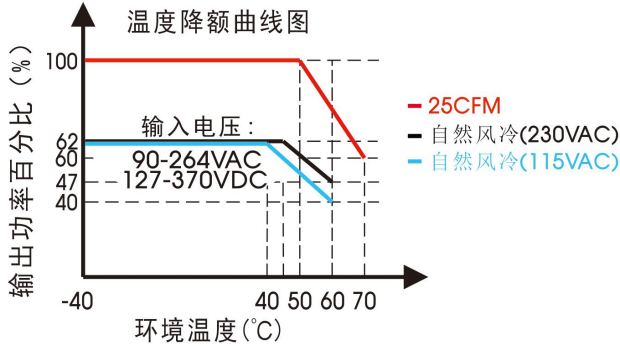
LOF450-20B12/15/18/19 (满载 400W 带 25CFM 风扇)
