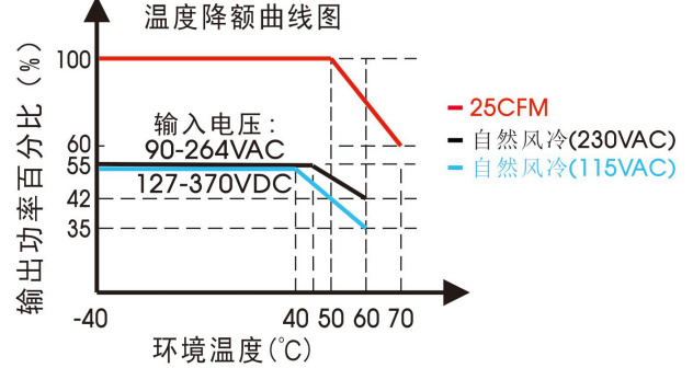
LOF450-20B24/27/36/48/54 (满载 450W 带 25CFM 风扇)
